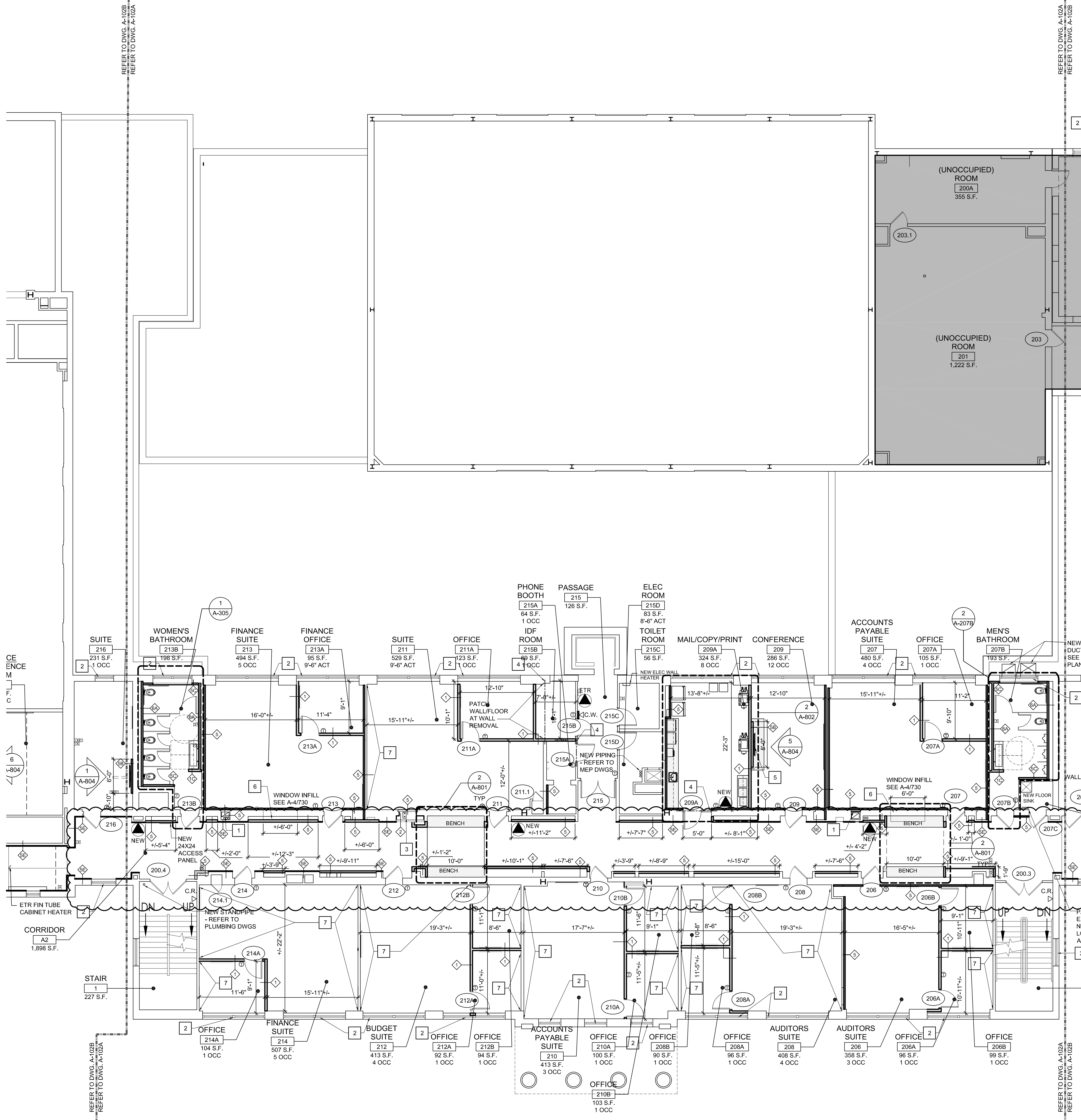
PARTIAL SECOND FLOOR PLAN AREA 'A' SCALE: 1/8" = 1'-0"
